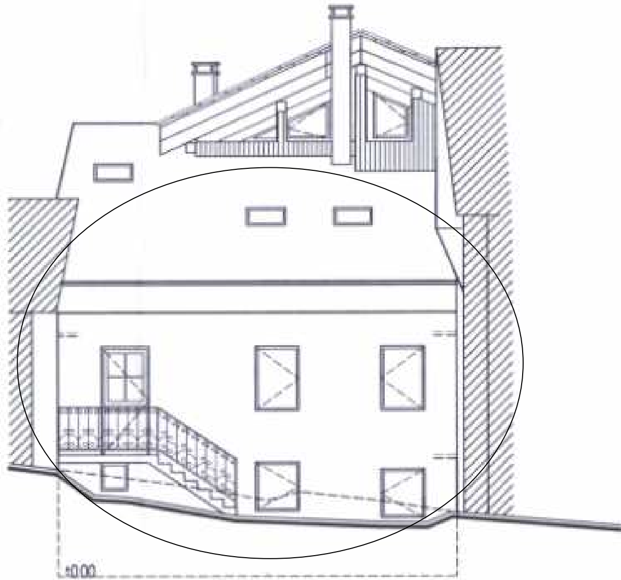
North-west elevation
